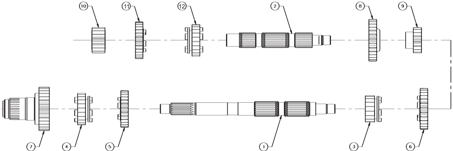
FIGURE 1 5-SPEED CLEAN-CUT GEARS
